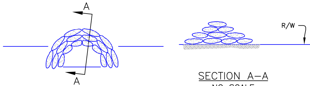
SANDBAG CHECKDAM NO SCALE
