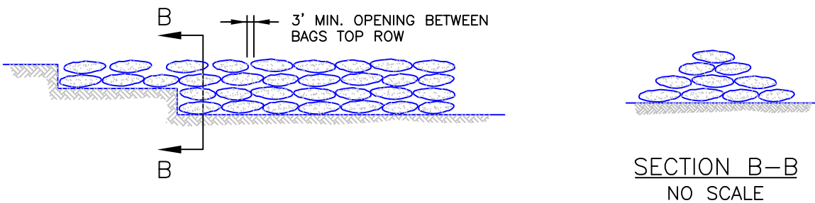
TYPICAL SANDBAG DETAIL NO SCALE
