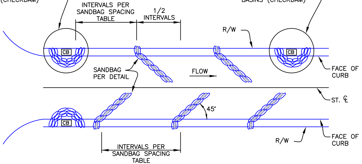
TYPICAL STREET SANDBAGGING DETAIL NO SCALE
