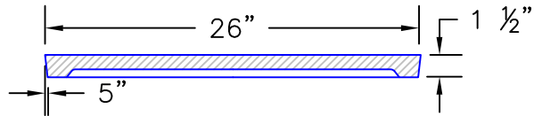
SECTION B-B (APPROX 144 LBS)
