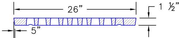
SECTION A-A (APPROX 175 LBS)
