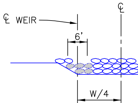
WEIR ELEVATION
