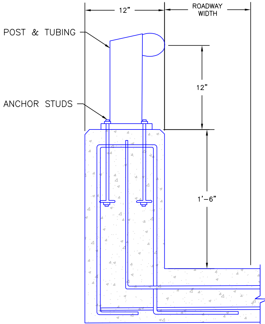
SECTION THROUGH PARAPET & RAIL
