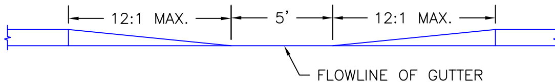
SECTION B-B
