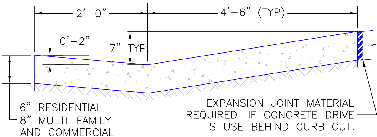
CROSS SECTION
