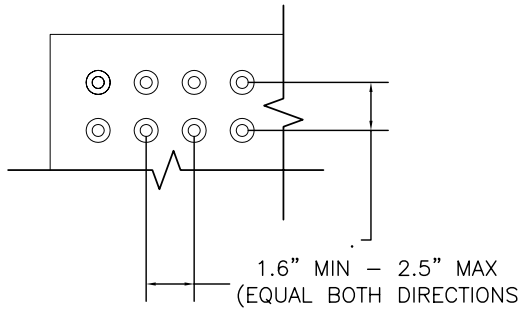
DOME SPACING
